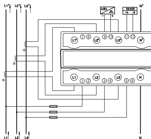
3 phase 4 wire input via CT
