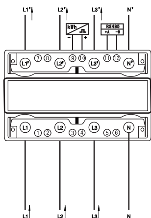
3 phase 4 wire direct input
